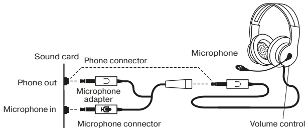
Fig. 1. Connection diagram
