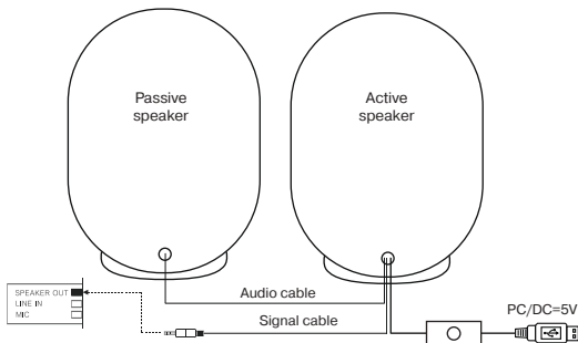
Fig. 2. Connection diagram
