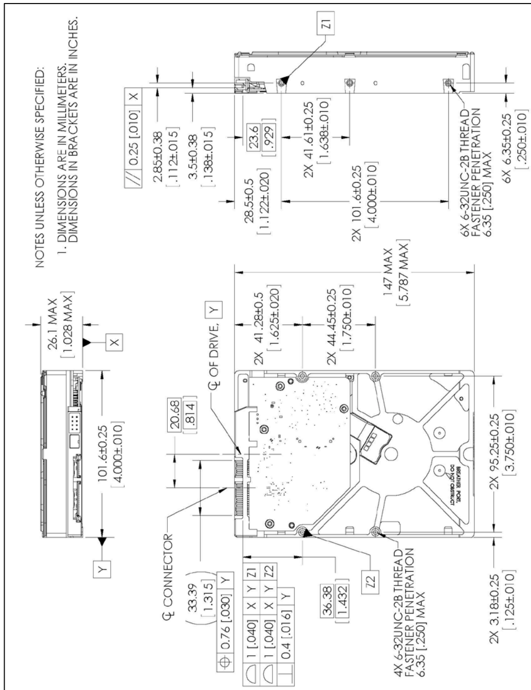
Figure 1 Mounting Dimensions
