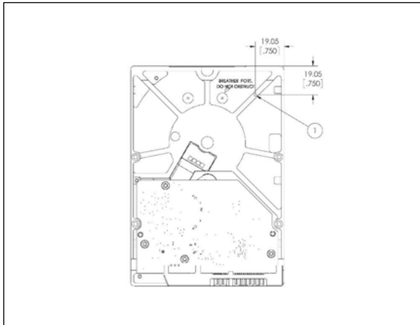
Figure 2 Drive Base Casting Thermocouple Location
