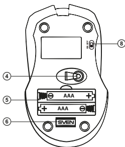
Fig. 2. Bottom view
