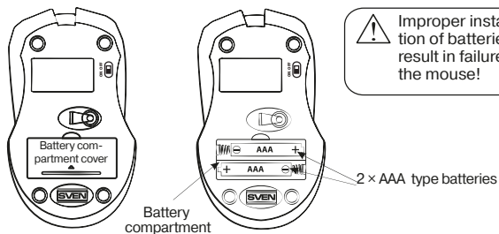
Fig. 4. Batteries installation
