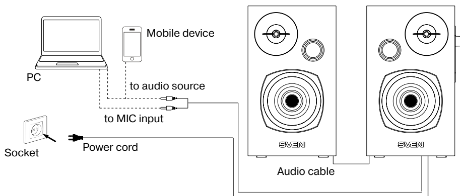
Fig. 2. Connection diagram
