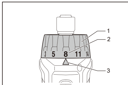
► 1. Adjusting ring 2. Graduation 3. Arrow
