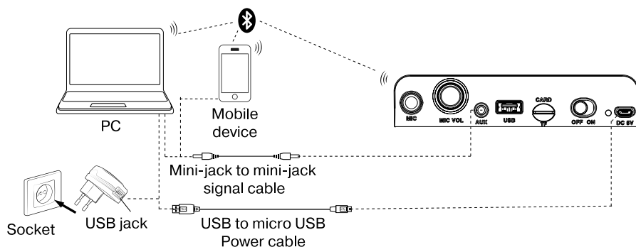
Fig. 3. Connection diagram
