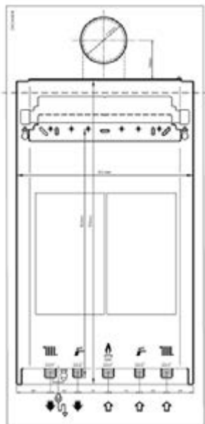
Figure 1 Installation scheme
