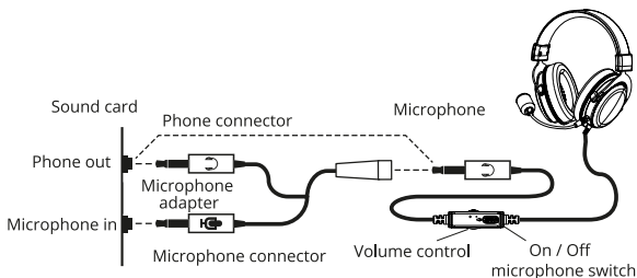
Fig. 2. Connection diagram
