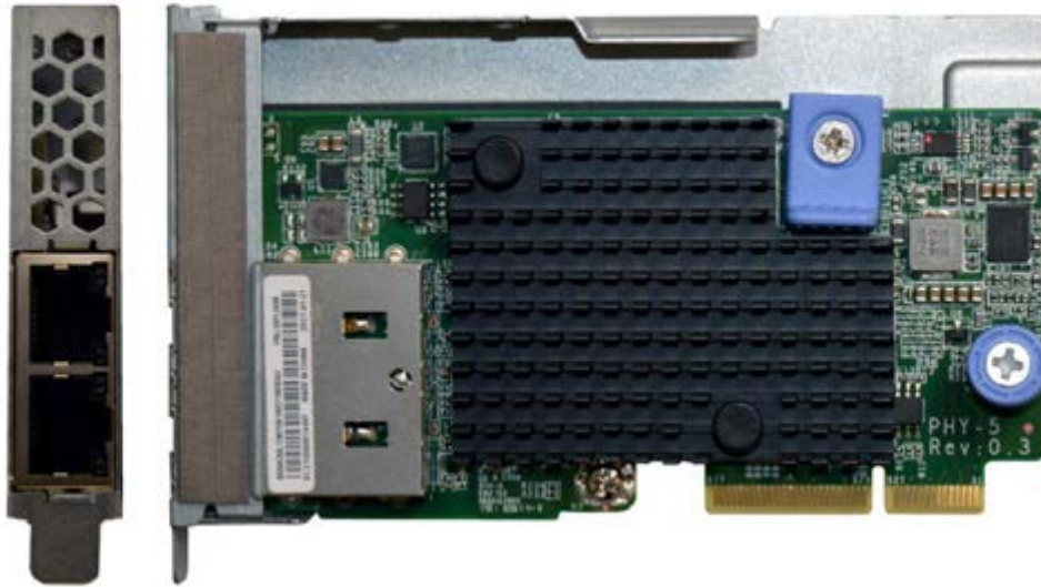
Figure 3. ThinkSystem 10Gb 2-port Base-T LOM
