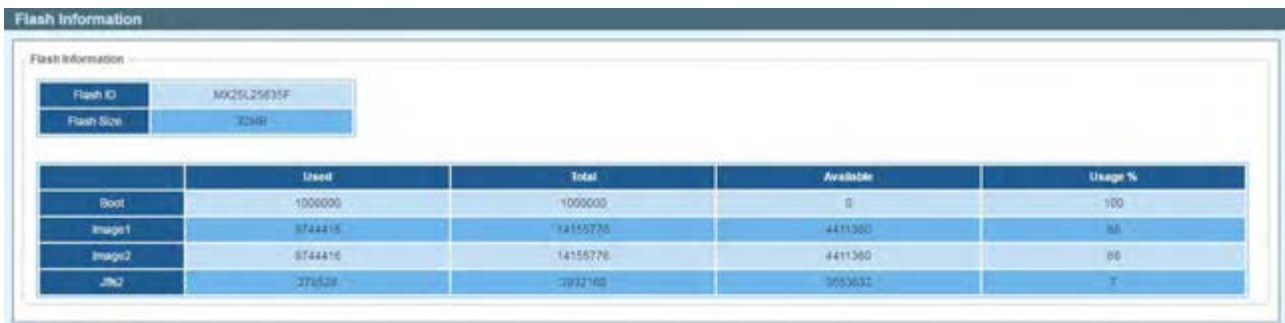
Figure 5.24 – Surveillance Mode &gt; Tools Menu &gt; Flash Information
