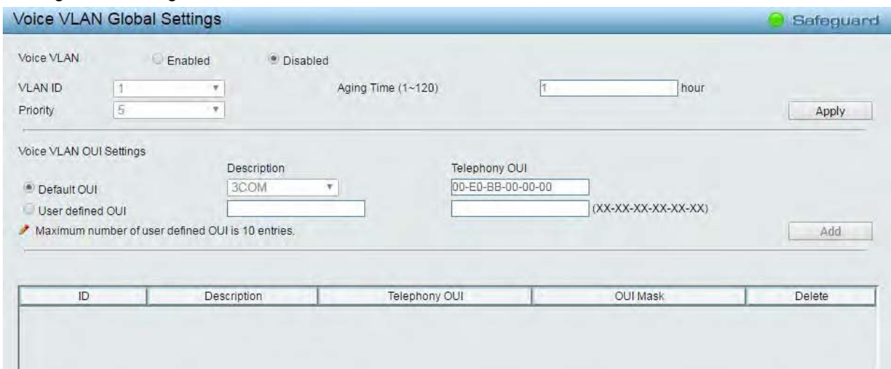
Figure 4.44 – VLAN > Voice VLAN > Voice VLAN Global Settings
