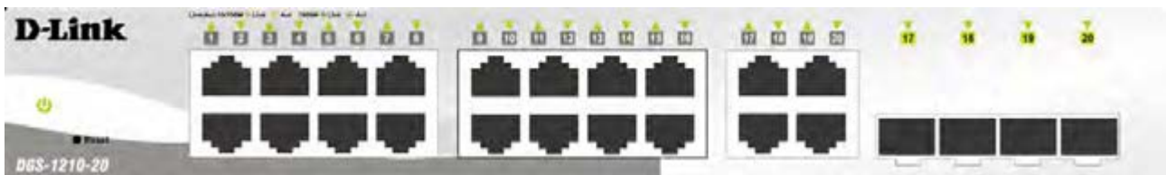
Figure 1.7 – DGS-1210-20 Front Panel
