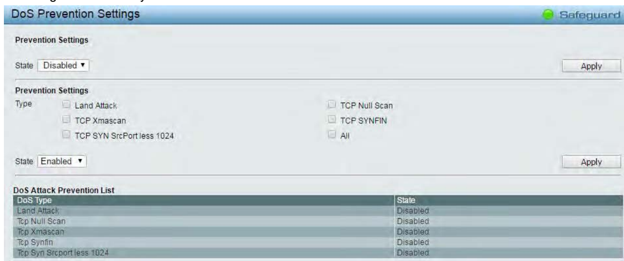
Figure 4.109 – Security > DoS Prevention Settings
