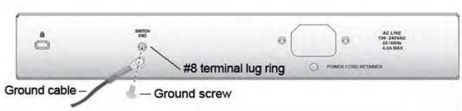
Figure 2.10 – Connect a Grounding Cable
