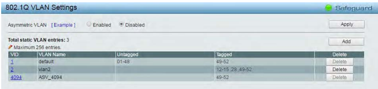
Figure 4.41 – Configuration > 802.1Q VLAN > Add VLAN
