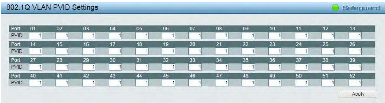
Figure 4.43 – Configuration > 802.1Q VLAN PVID
