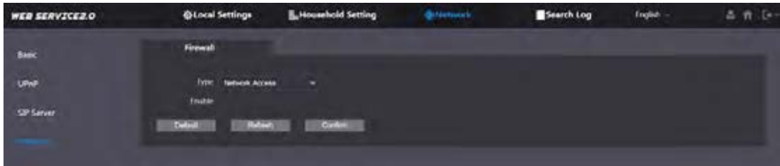
Figure 6-4 Firewall
