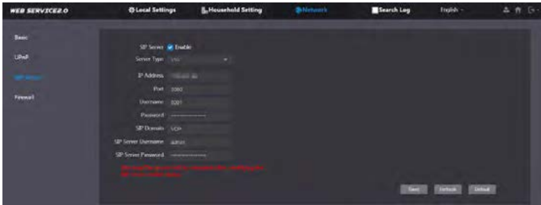
Figure 6-3 SIP Server
