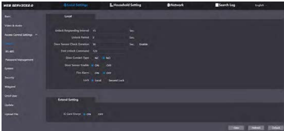
Figure 4-3 Local
