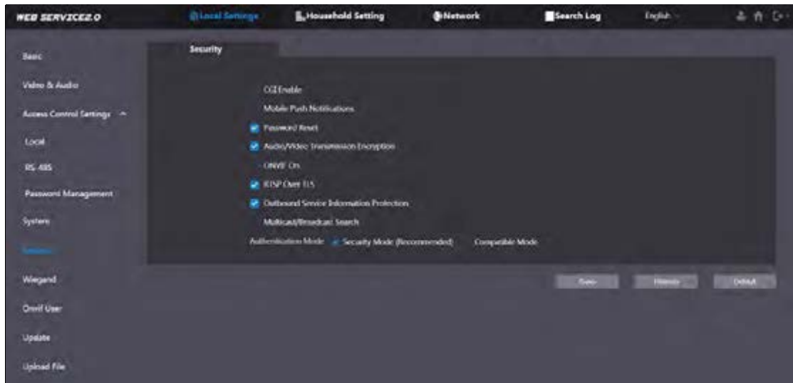
Figure 4-7 Security
