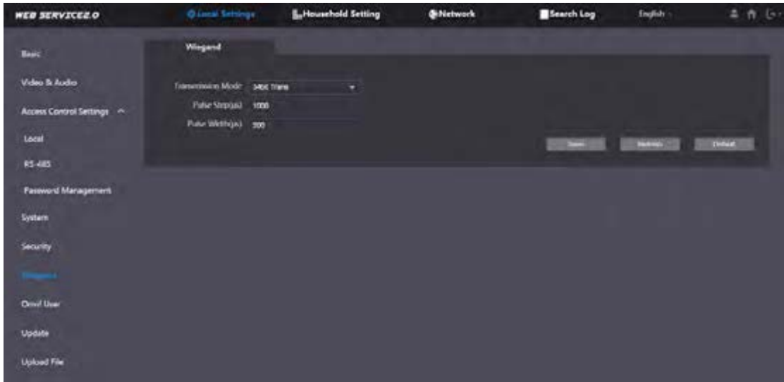
Figure 4-8 Wiegand
