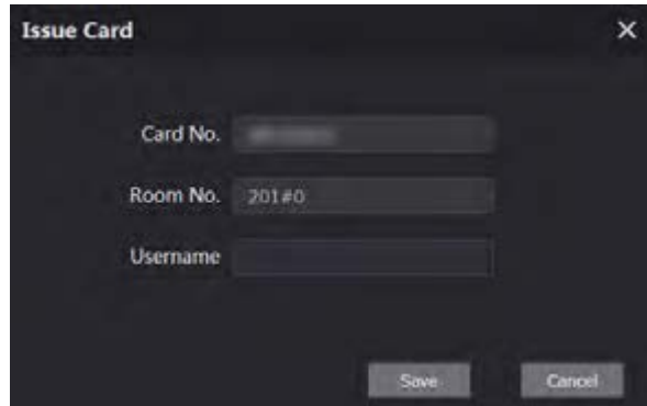
Figure 5-11 Issue card
