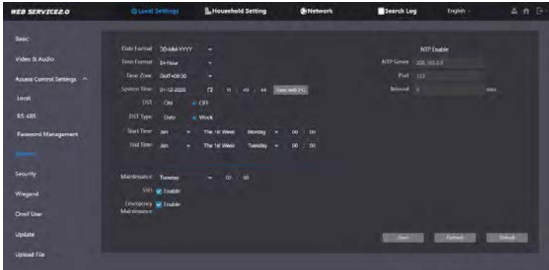
Figure 4-6 System
