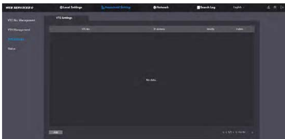
Figure 5-14 VTS management
