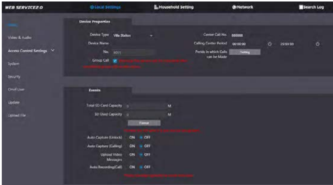
Figure 4-1 Basic
