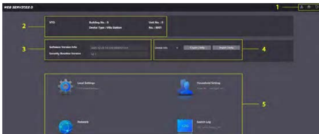
Figure 3-1 Main interface
