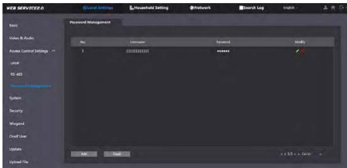
Figure 4-5 Password management
