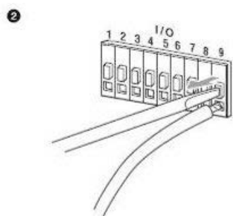
Figure 8-5 Remove cable
