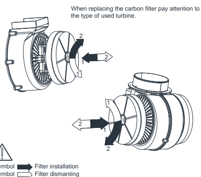
Fig. 10 Replacing the carbon filter.
