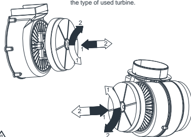
Fig. 10 Replacing the carbon filter.
