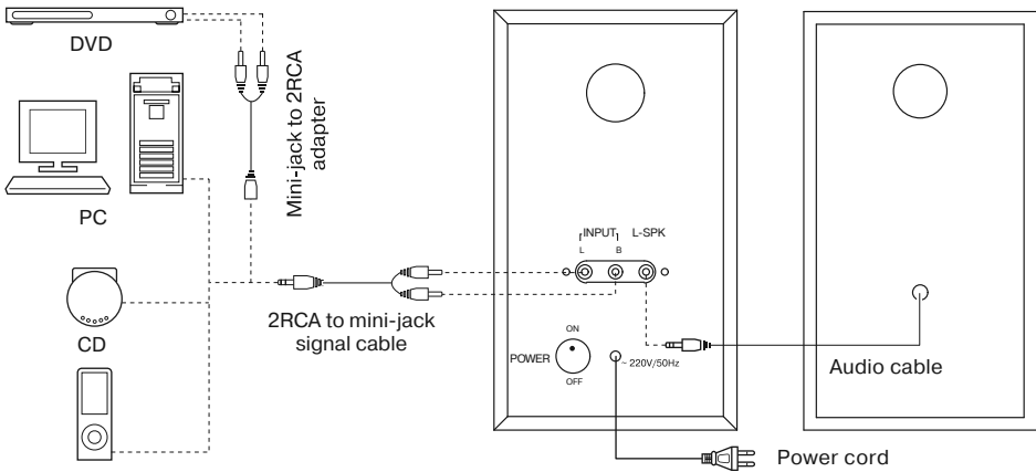
Fig. 2. Connection diagram
