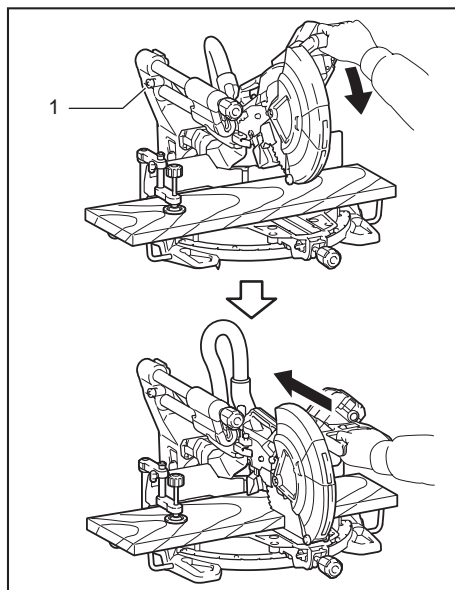
▶ 1. Stopper pin
