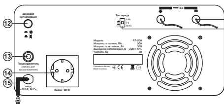
Fig. 3. Rear panel of RT-500
