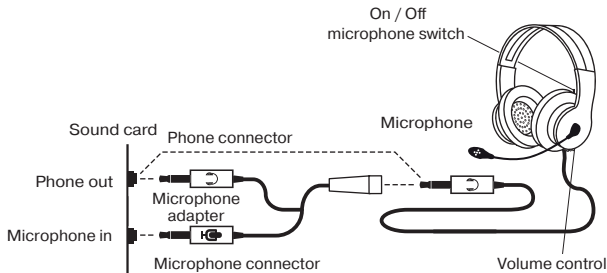
Fig. 1. Connection diagram
