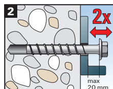
2 Therefore the screw may be tightened to a maximum of 20 mm of the surface of the initial fixture. The total permissible thickness of shims added during the adjustment process is 10 mm.
