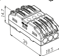
plc-smk-423
