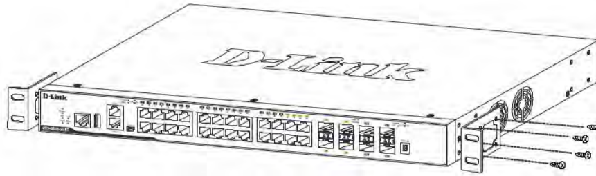
Figure 2 — Attaching rack-mount brackets to the Switch
