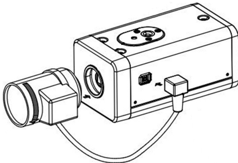
Figure 9-1 Lens installation (1)
