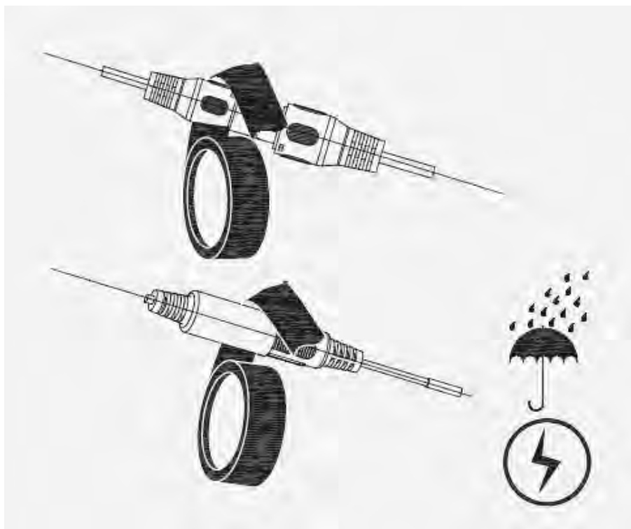
Figure 11-2 Waterproof measures
