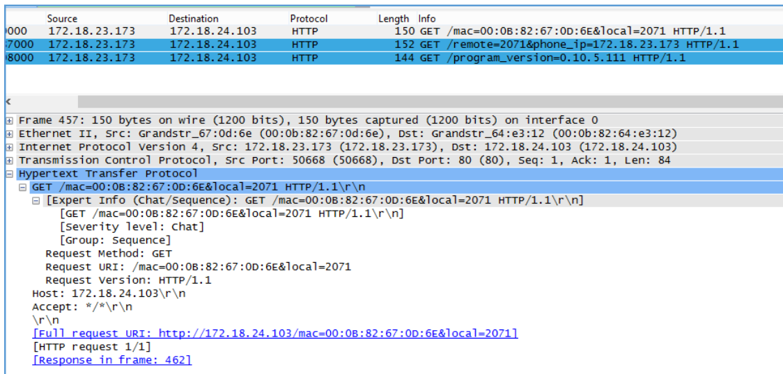
Figure 10: Action URL Packet
