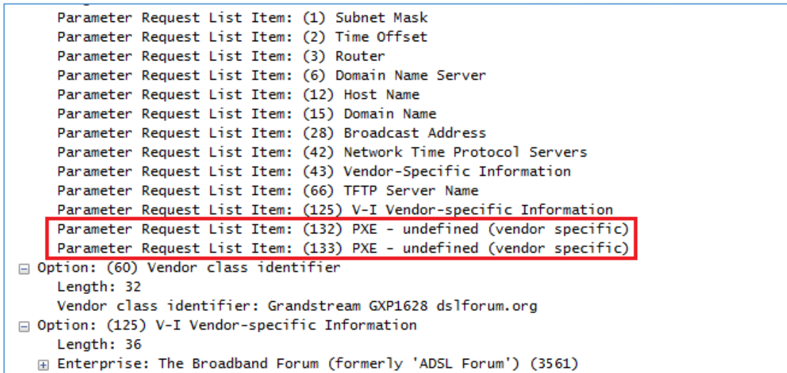
Figure 5: DHCP Option 132 & 133
