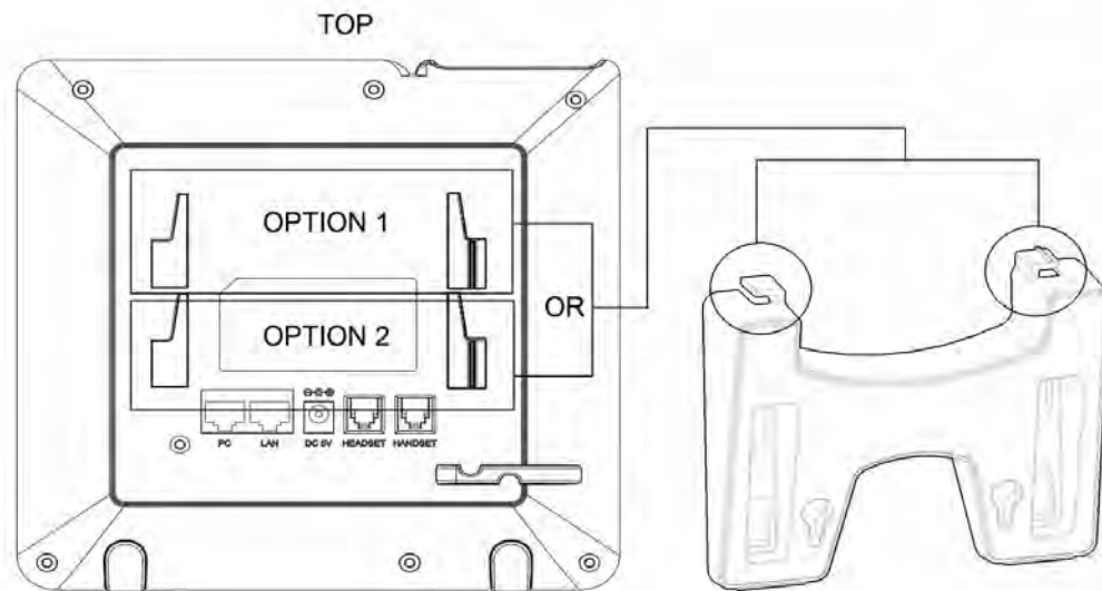
Figure 2: GXP16xx Stand Installation
