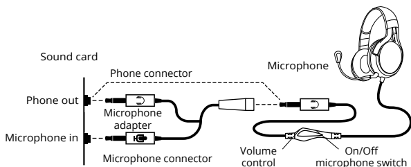
Fig. 2. Connection diagram
