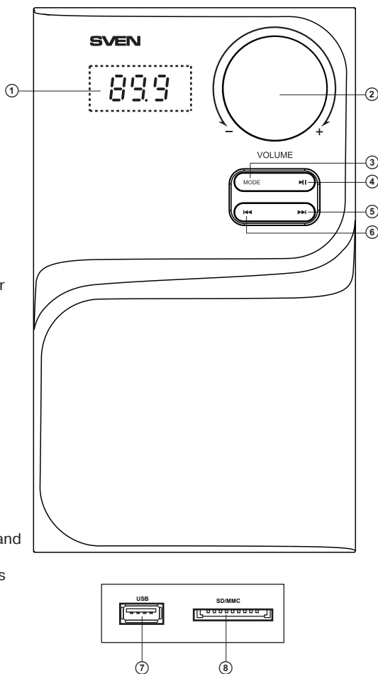
Fig. 1. Subwoofer control panel
