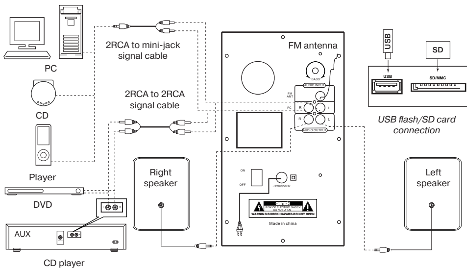
Fig. 4. Connection diagram
