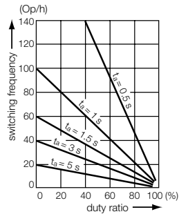
Intermittent periodic duty, t_a : Motor starting time
