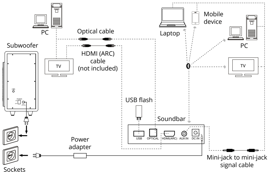
Fig. 4. Connection diagram
