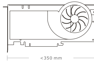
VGA (Add-on card) Length Limitation
