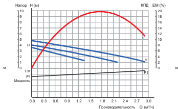
VCP 32-40G
