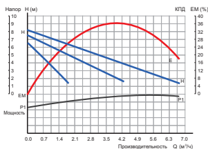
VCP 25-80G
