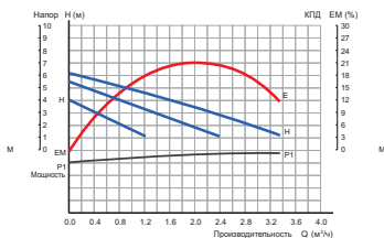
VCP 32-80G
