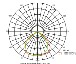
LED-TV-400W
