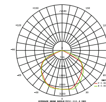
LED-TV-600W
