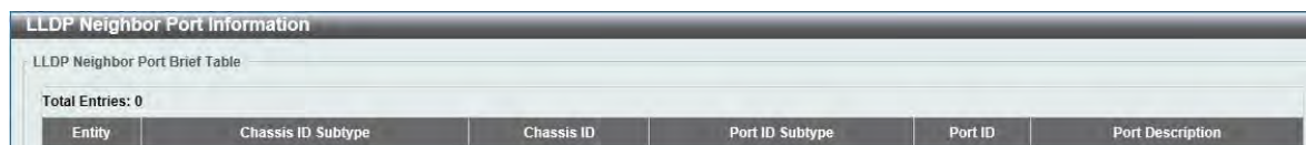
Figure 7-32 LLDP Neighbor Port Information window
