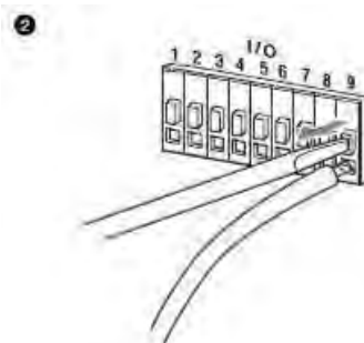
Figure 8-5 Remove cable
