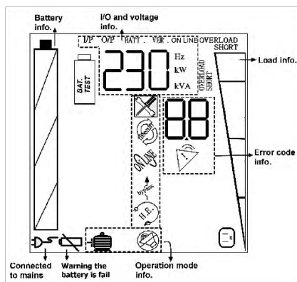
Tower Display
