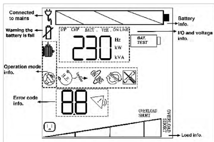
Rack Display
