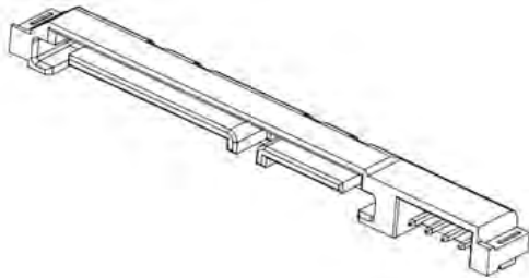
SATA plug connector overview (MG08ACA16T / 14T) (MG08ACP16T)
