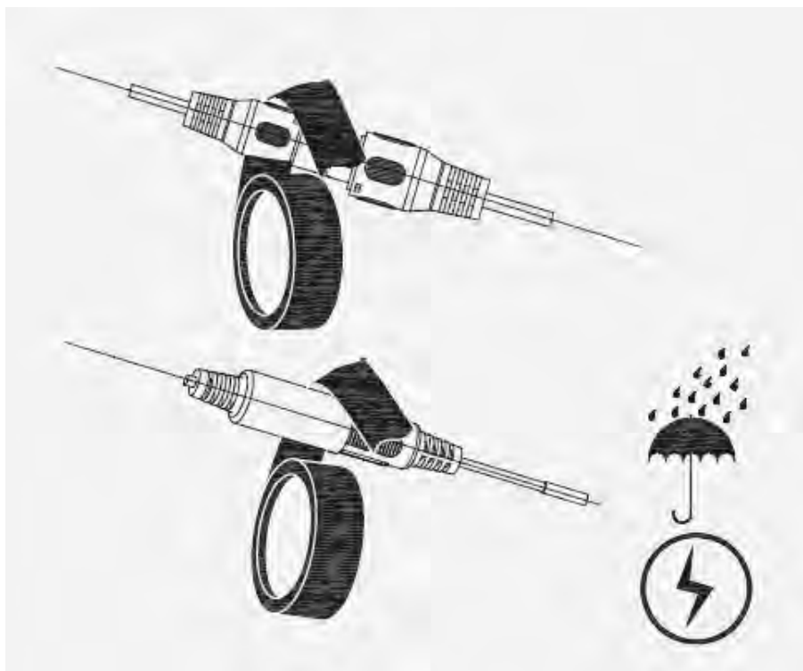
Figure 11-2 Waterproof measures
