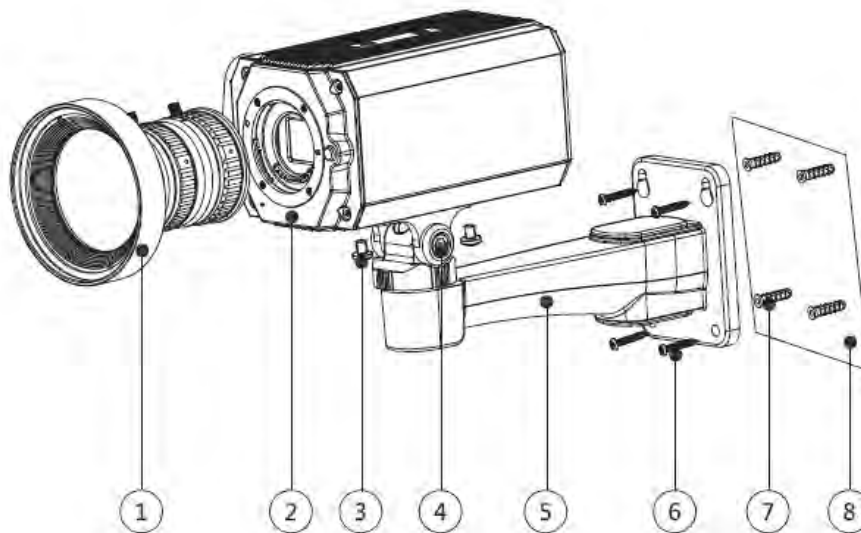
Figure 8-6 Device components
