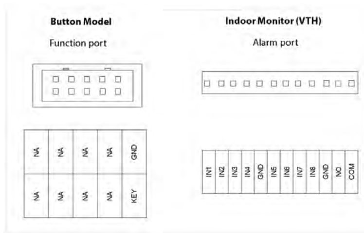
Figure 12-2 Cable connection
