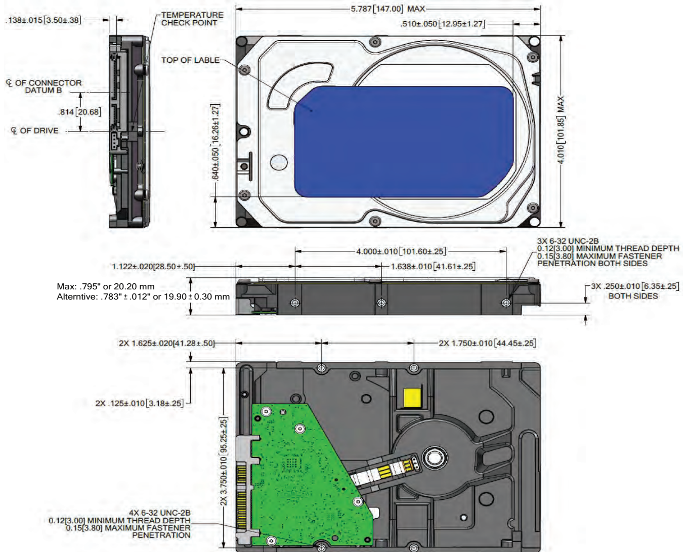
Figure 2 Mounting dimensions (1 and 2-disk models)
