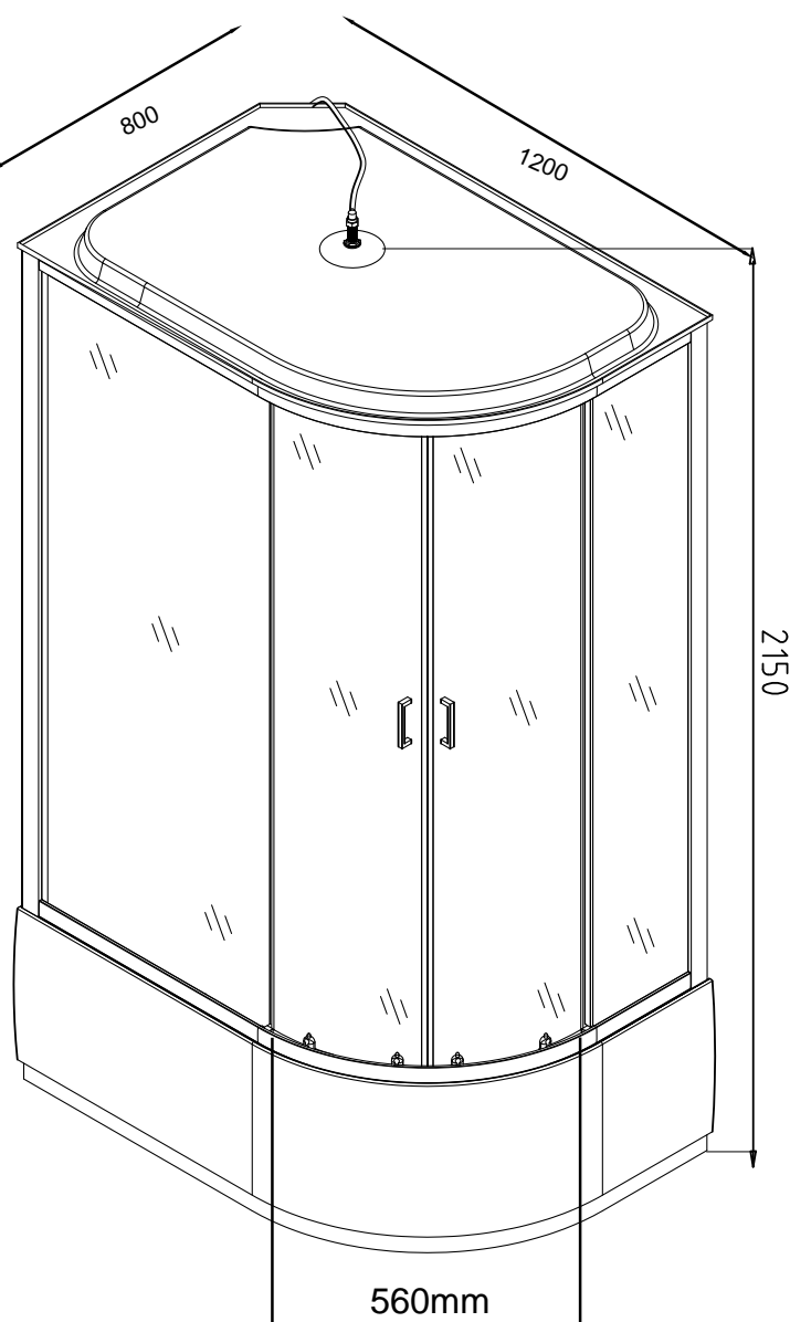
SC-1200QL 1200x800x2150(243331)
