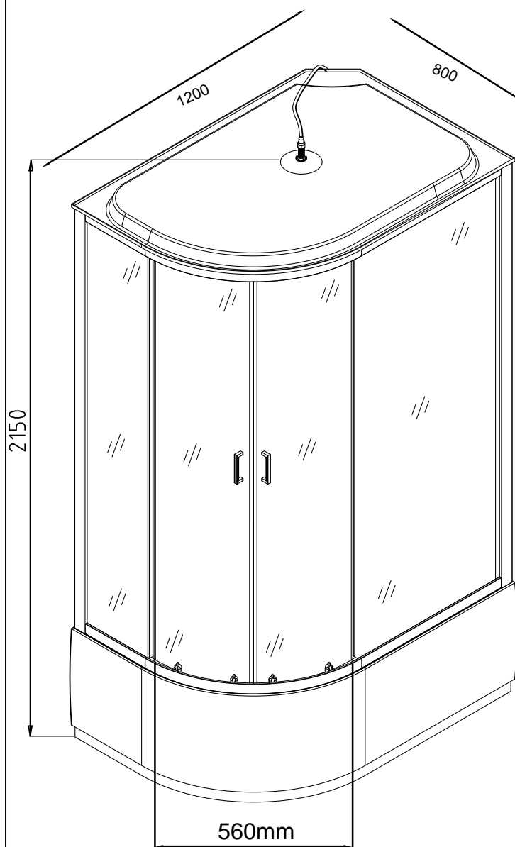
SC-1200QR 1200x800x2150(243330)
