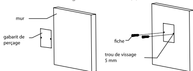
Image 7-4 Installation (1)
