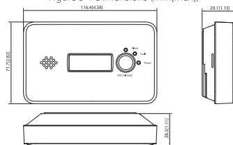
Figure 3-1 Dimensions (mm[inch])
