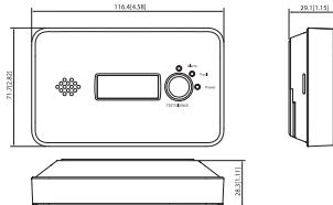
Image 3-1 Dimensions (mm[inch])
