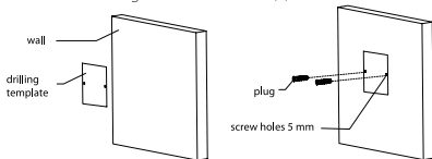
Figure 7-4 Installation (1)
