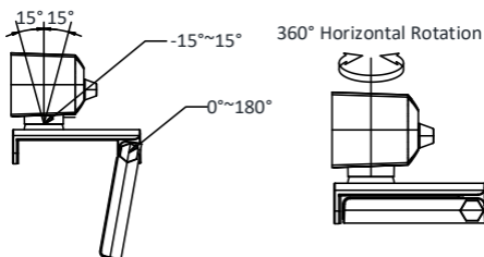
Figure 2-1 Angle Adjustment
