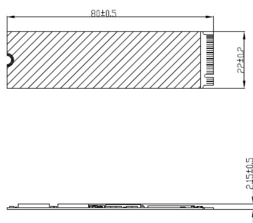
<Without heatsink>
