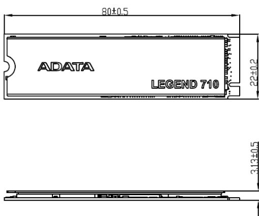
<With heatsink>
