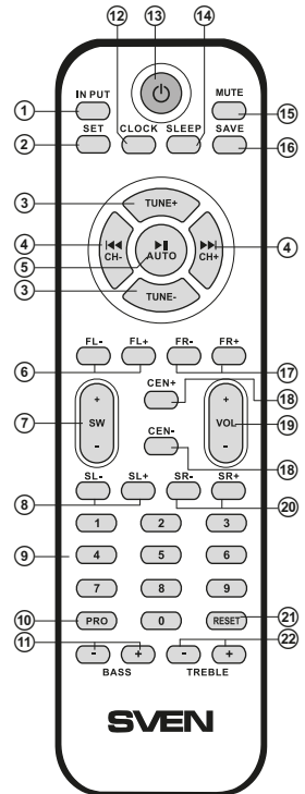
Fig. 4. Remote control
