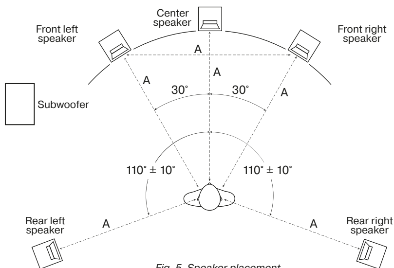
Fig. 5. Speaker placement
