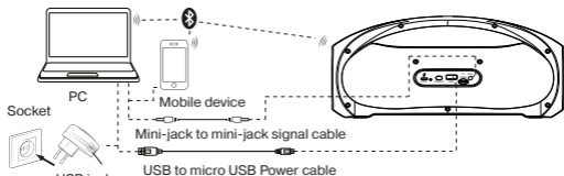
Fig. 4. Connection diagram
