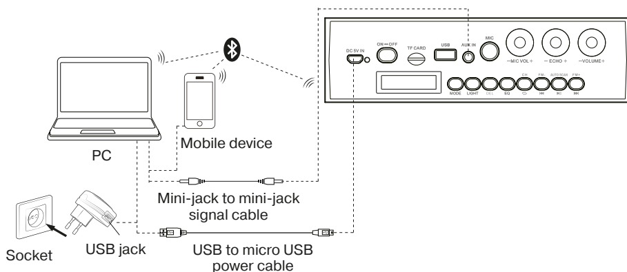
Fig. 2. Connection diagram
