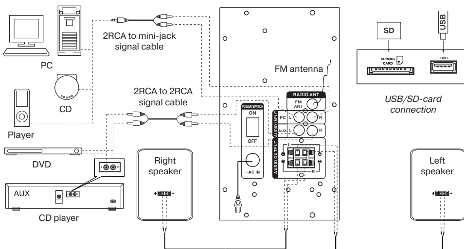
Fig. 4. Connection diagram
