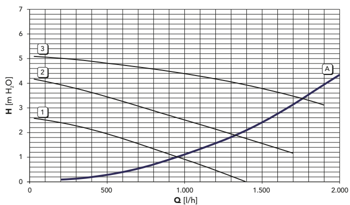
Circulating pump head / pressure losses DIVAtech D HF24
