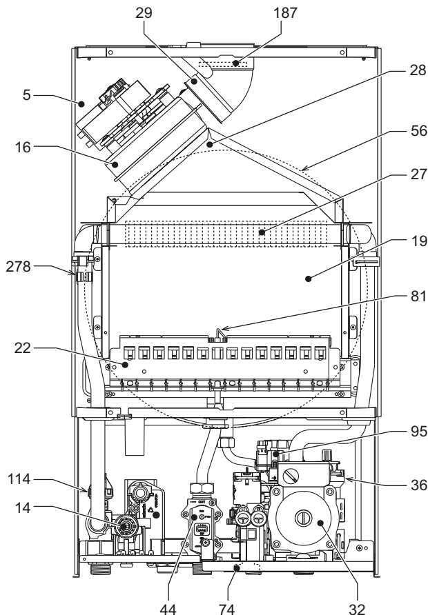
fig. 28- General view - DIVAtech D HF32
