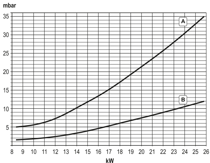
Pressure - power diagrams DIVAtech D HF24
