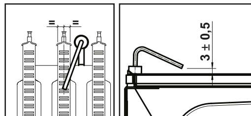
fig. 20 - Electrode positioning
