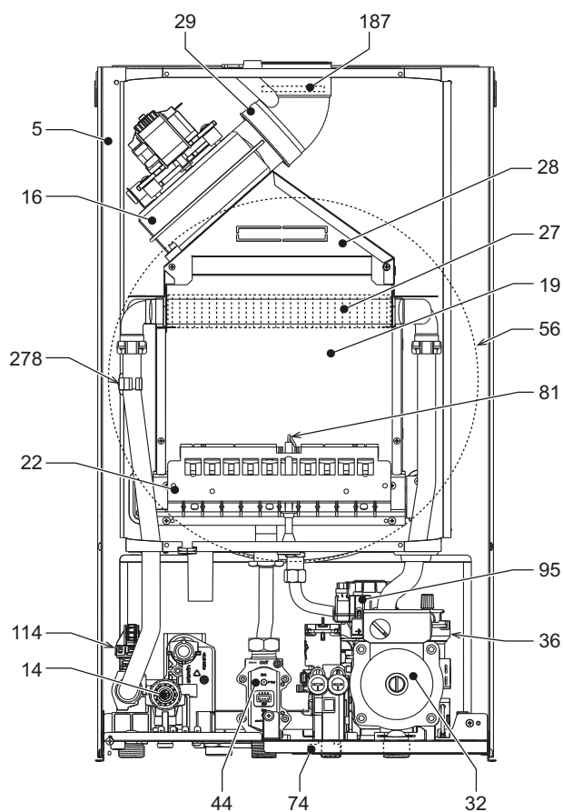
fig. 27- General view - DIVAtech D HF24
