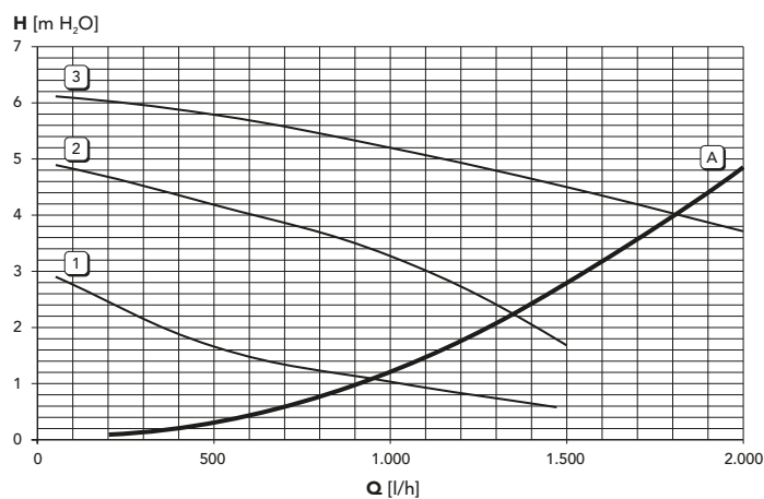
Circulating pump head / pressure losses DIVAtech D HF32
