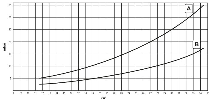
Pressure - power diagrams DIVAtech D HF32
