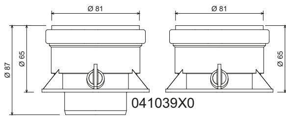
fig. 18 - Starting accessory for separate ducts
