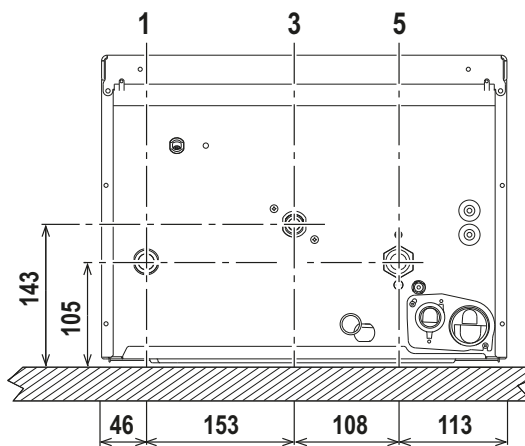
fig. 12 - Plumbing connections
