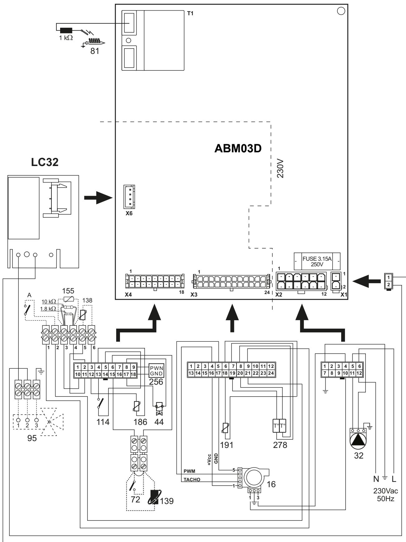
fig. 29 - Wiring diagram
