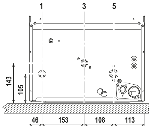
fig. 12 - Raccordements hydrauliques
