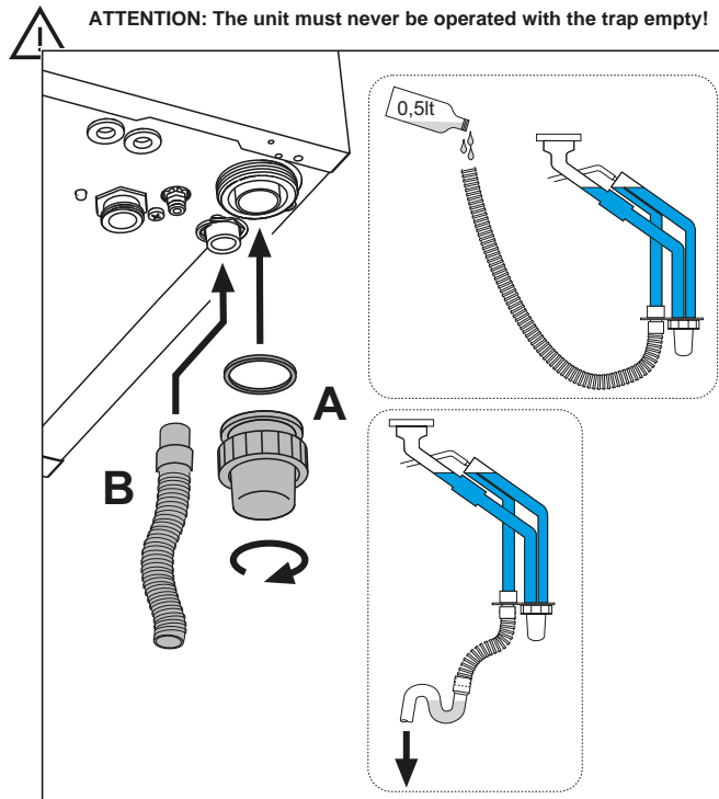
fig. 20 - Condensate outlet connection
