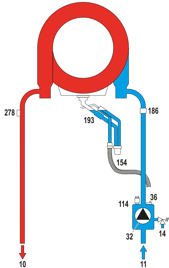
fig. 28 - Hydraulic circuit
