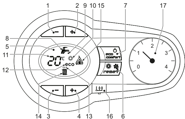
fig. 1 - Control panel
