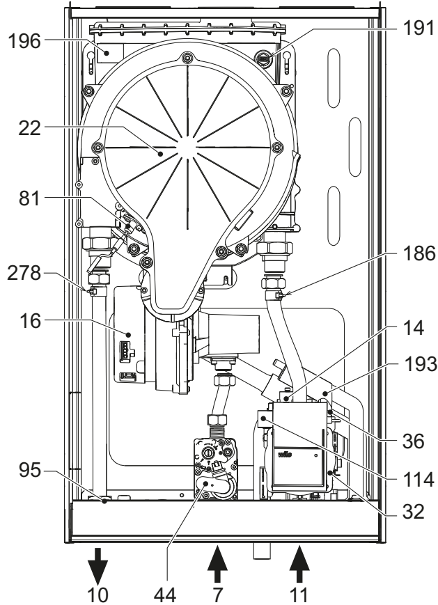
fig. 26 - General view
