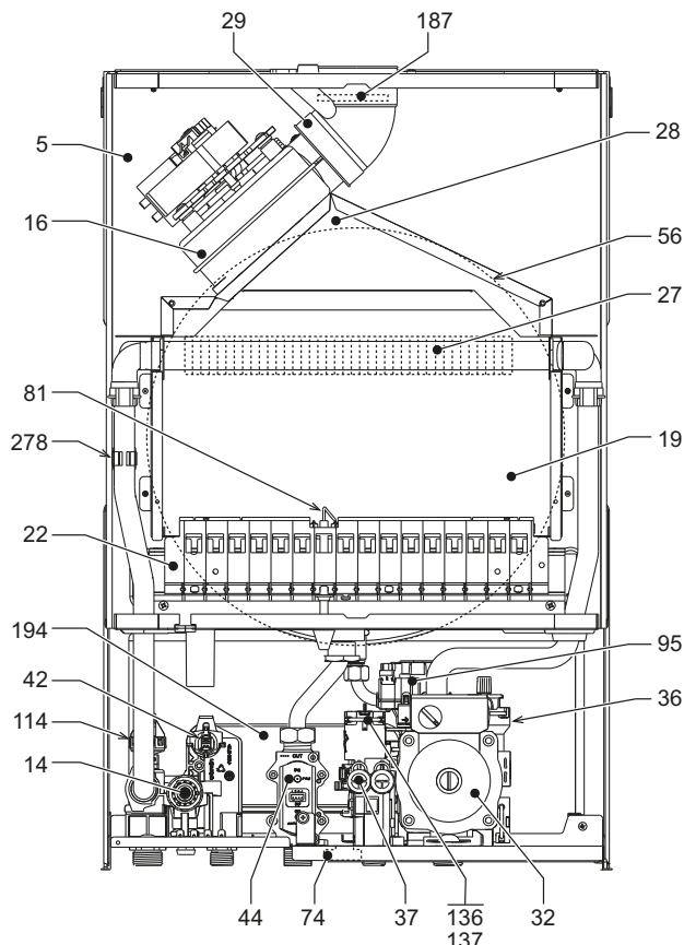
fig. 29- General view - DIVAtech D F37
