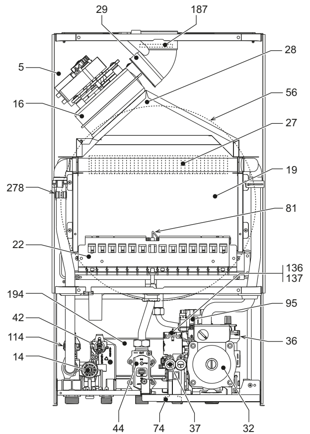
fig. 28- General view - DIVAtech D F32
