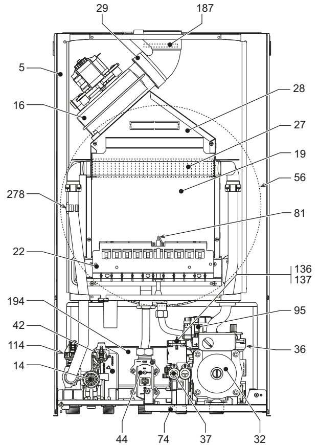
fig. 27- General view - DIVAtech D F24
