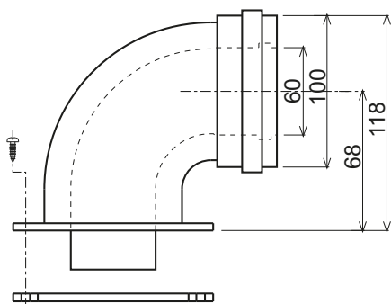
fig. 12 - Starting accessory for coaxial ducts
