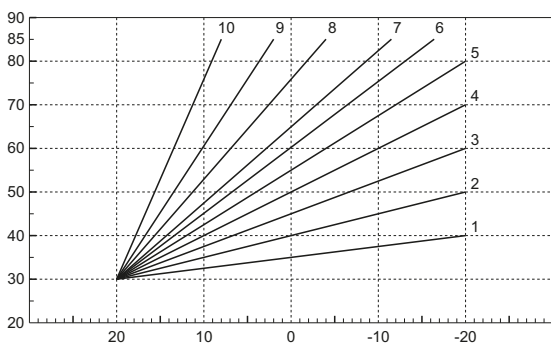
fig. 6 - Compensation curves
