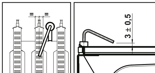
fig. 19 - Electrode positioning
