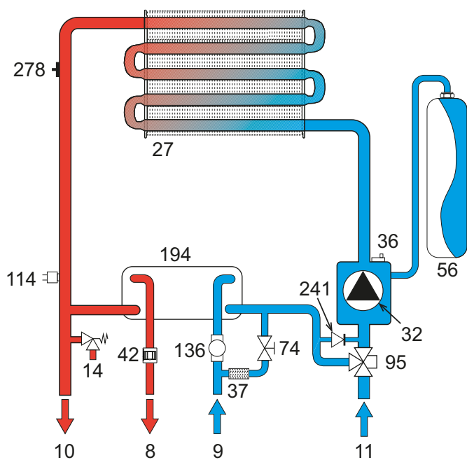
fig. 30- Heating circuit
