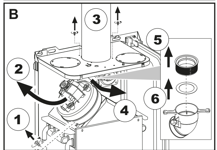
A Baffle replacement with boiler not installed B Baffle replacement with boiler and fume ducts already installed
