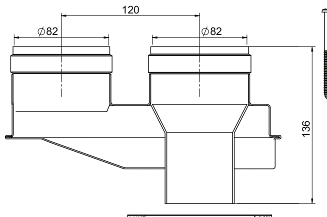
fig. 14 - Starting accessory for separate ducts code 010031X0
