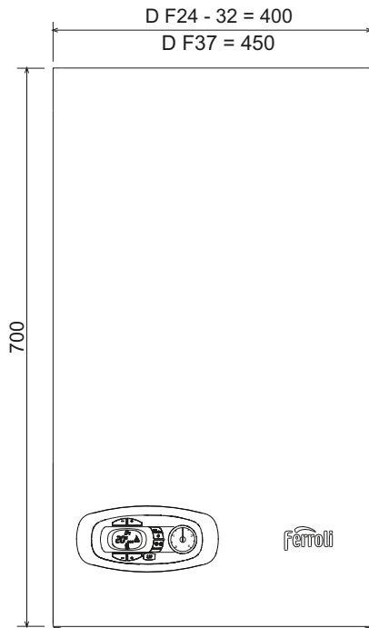
fig. 20- Front view
